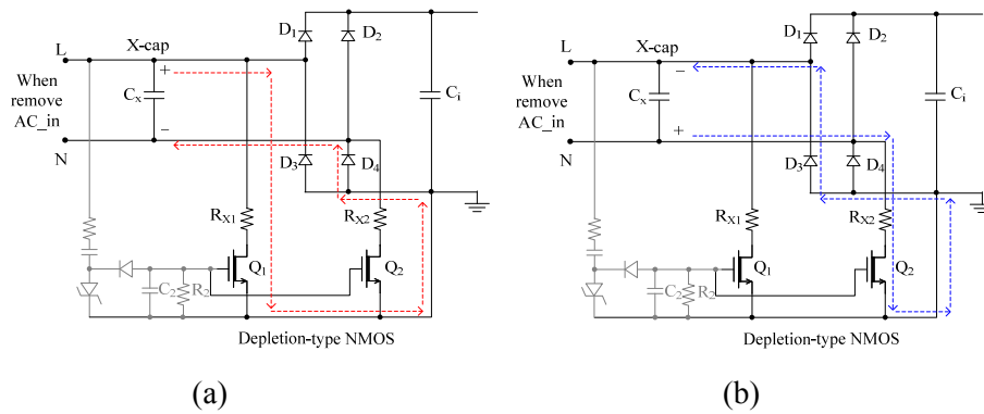
Fig. 3. Two discharge path when remove AC power.
